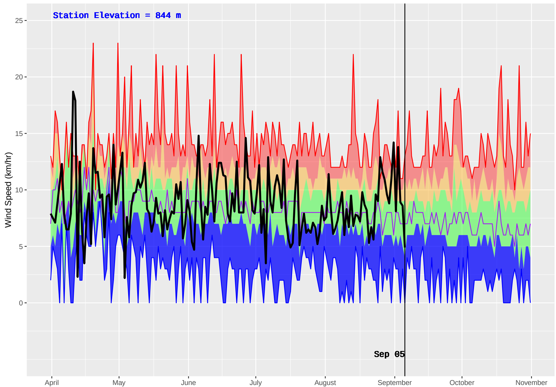
GANOKWA (182) : Historical (1993–2016) and Current (2018) Daily Wind Speed
